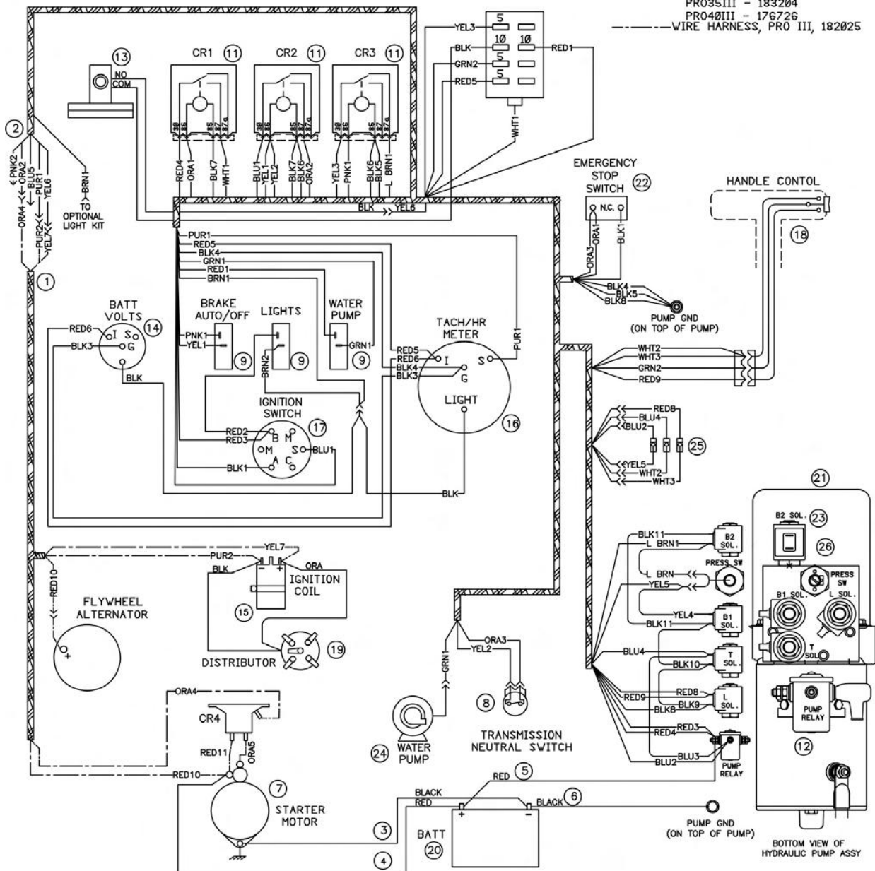
DIAG. LOC. PART NO. QTY REQ DESCRIPTION DIAG. LOC. PART NO. QTY REQ DESCRIPTION 1 183204 1 Wiring Harness, Engine 14 166438 1 Gauge, Battery Volts 2 182025 1 Wiring Harness, Cowl 15 ----- 1 Coil, Ignition (Wisconsin #YF388) 3 163179 1 Cable, Battery, Negative 40" 16 163665 1 Gauge, Tach. / Hour Meter 4 163180 1 Cable, Battery, Positive 52" 17 166707 1 Switch, Ignition 5 176838 1 Cable, Battery, Positive Hyd. 8" 18 183135 1 Handle, Trans/Lift Control 6 176714 1 Cable, Battery, Negative Hyd. 13" 19 ----- 1 Distributor (Wisconsin #YF50AS1) 7 ----- 1 Starter (Wisconsin #YB53A) 20 163121 1 Battery, 12 Volt 8 166447 1 Switch, Neutral Safety 21 176992 1 Hydraulic Pump Assembly 9 166711 3 Switch, Rocker 22 176383 1 Emergency Stop Switch 10 166622 1 Block, Fuse 23 166594 4 Coil - 12V DC 11 166708 3 Relay, N.O. N.C. 24 164977 1 Water Pump (Optional) 12 166121 1 Solenoid Relay 25 182036 1 Diode Assembly, Hyd. Brake 13 047136 1 Water Safety Switch 26 183007 1 Pressure Switch
